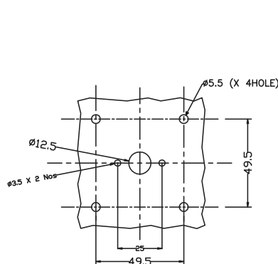
PANEL CUTOUT
